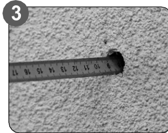
3 Insert tube, or measure depth of hole from finished render back to the original substrate. Allow for the depth of the WL bracket and an allowance of 4mm for the neoprene washer to compress and provide a seal when installed.
