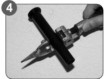
4 Cut tube to length using pipe cutter ensuring an allowance has been made for the dept of the plate.
